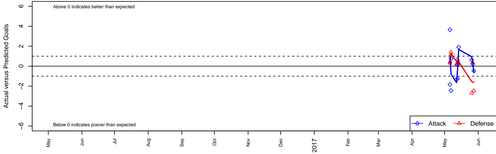
CGA Academy SC Elite B98 Dots are actual minus expected GF (blue circles) and GA (red triangles). Blue line is smoothed change in attack strength. Red is smoothed change in defense strength.
